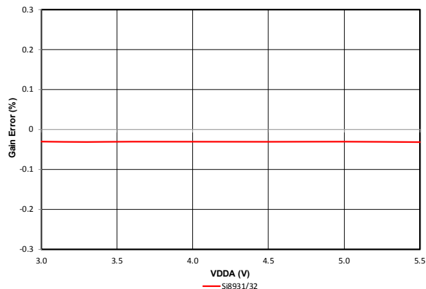
Figure 4.21. Gain Error (%) vs. VDDA Supply (V)
