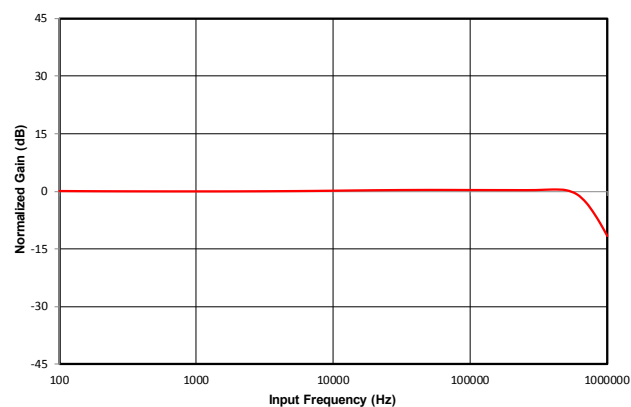
Figure 4.25. Amplifier Bandwidth
