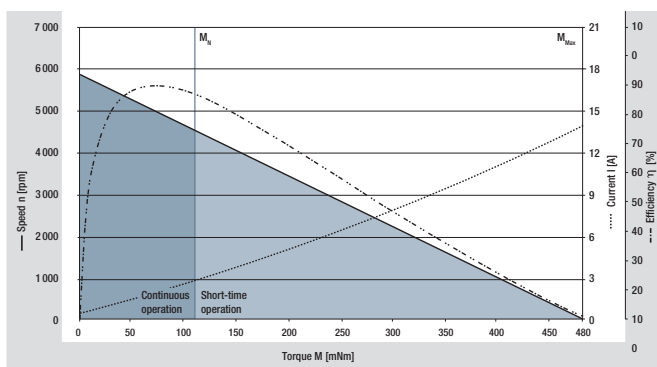
A ECI-42.20, 24 V (at 25 °C)
