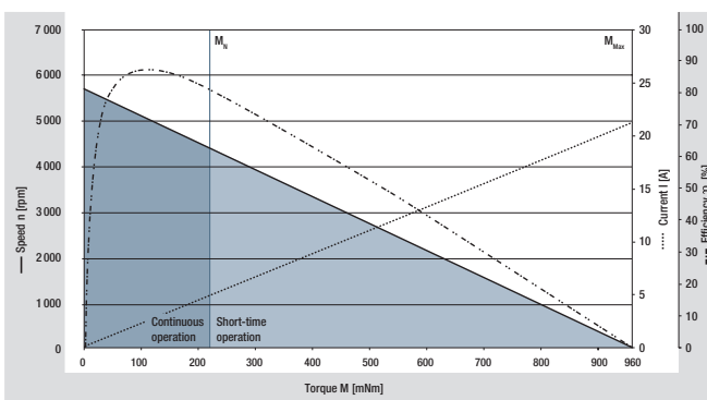
B ECI-42.40, 24 V (at 25 °C)
