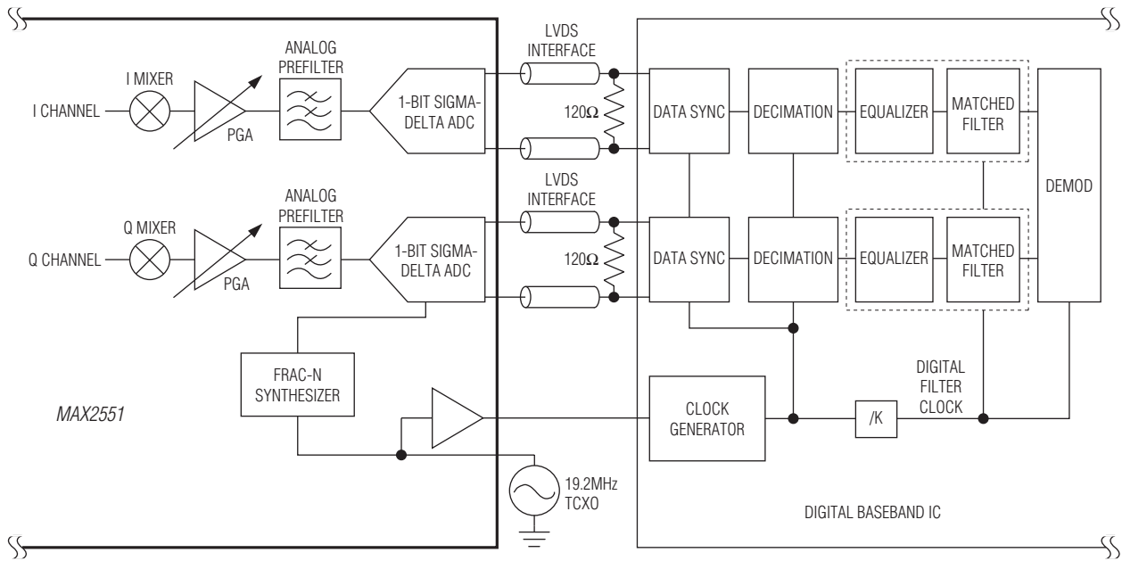
Figure 1. Digital Baseband Receiver Interface
