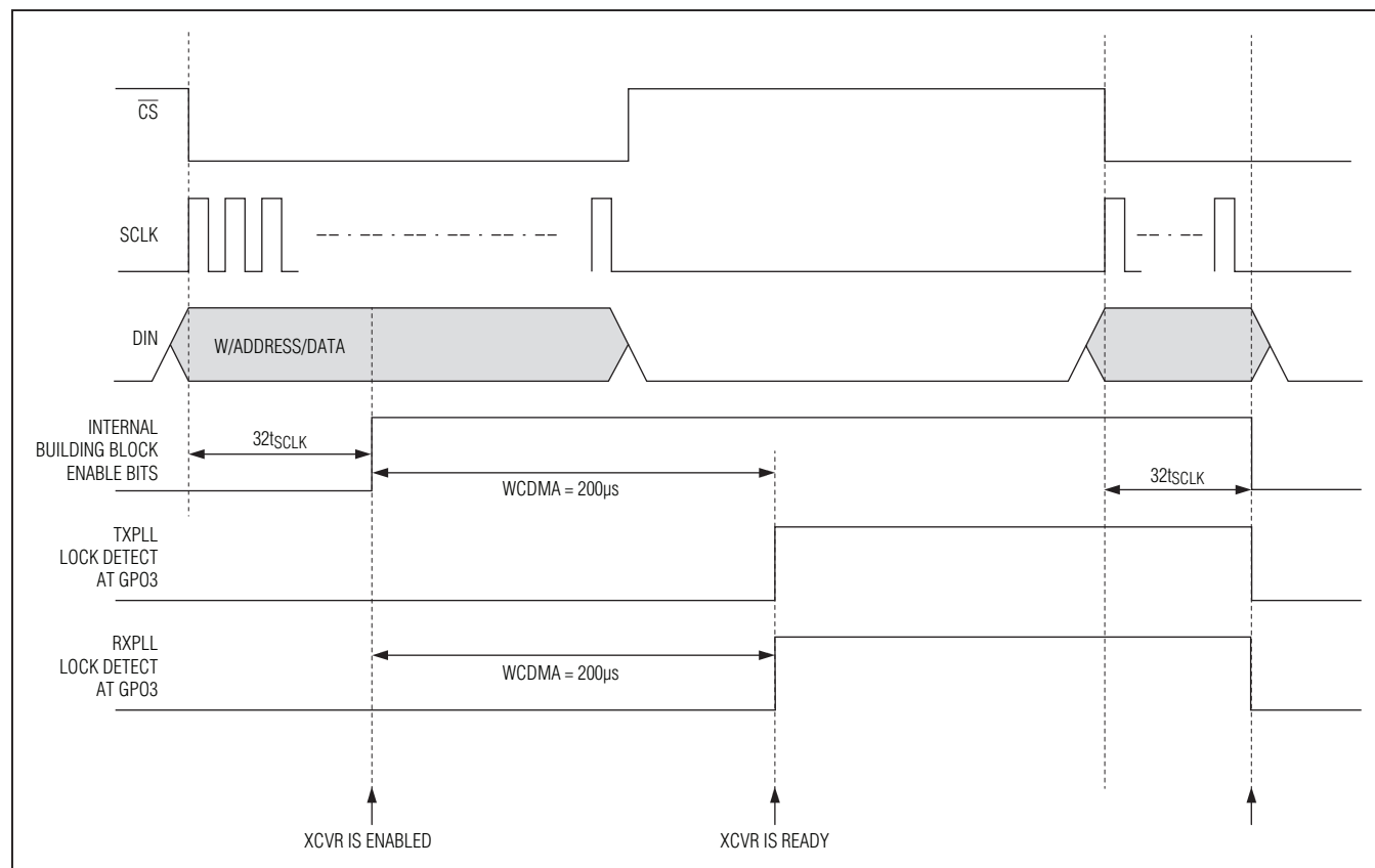
Figure 3. POR PLL Lock-Detect Time
