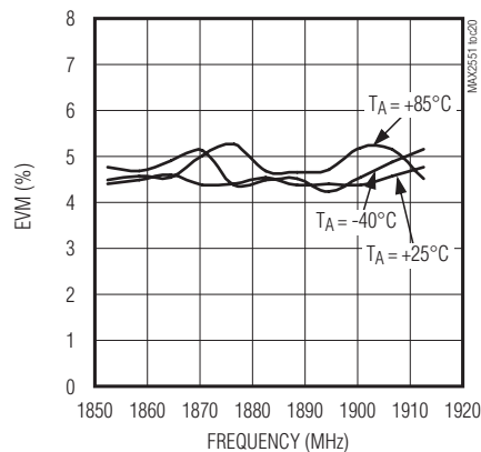
RXIN1 EVM vs. FREQUENCY
