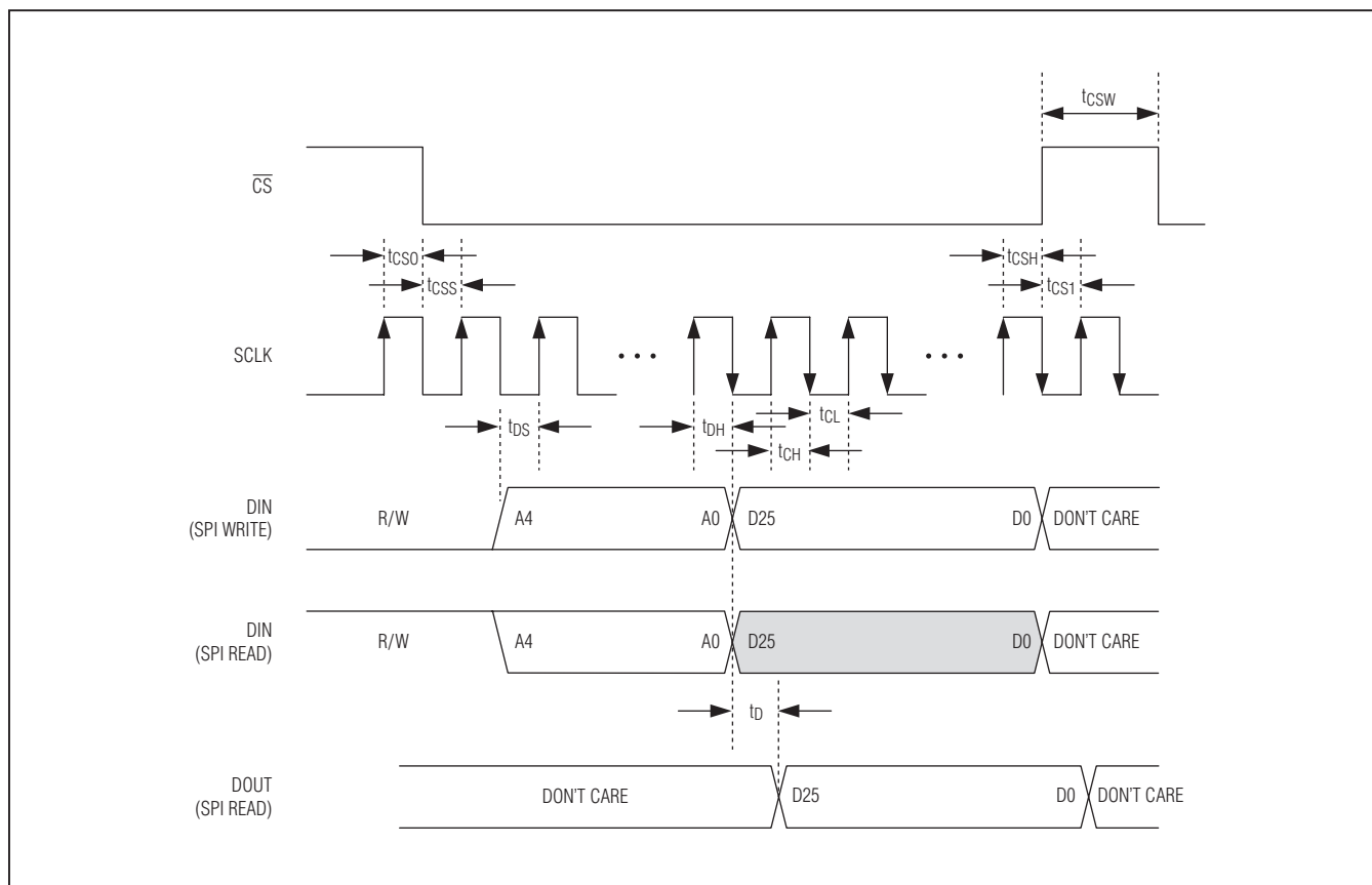
Figure 4. SPI Timing
