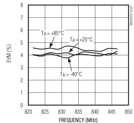
RXIN3 EVM vs. FREQUENCY
