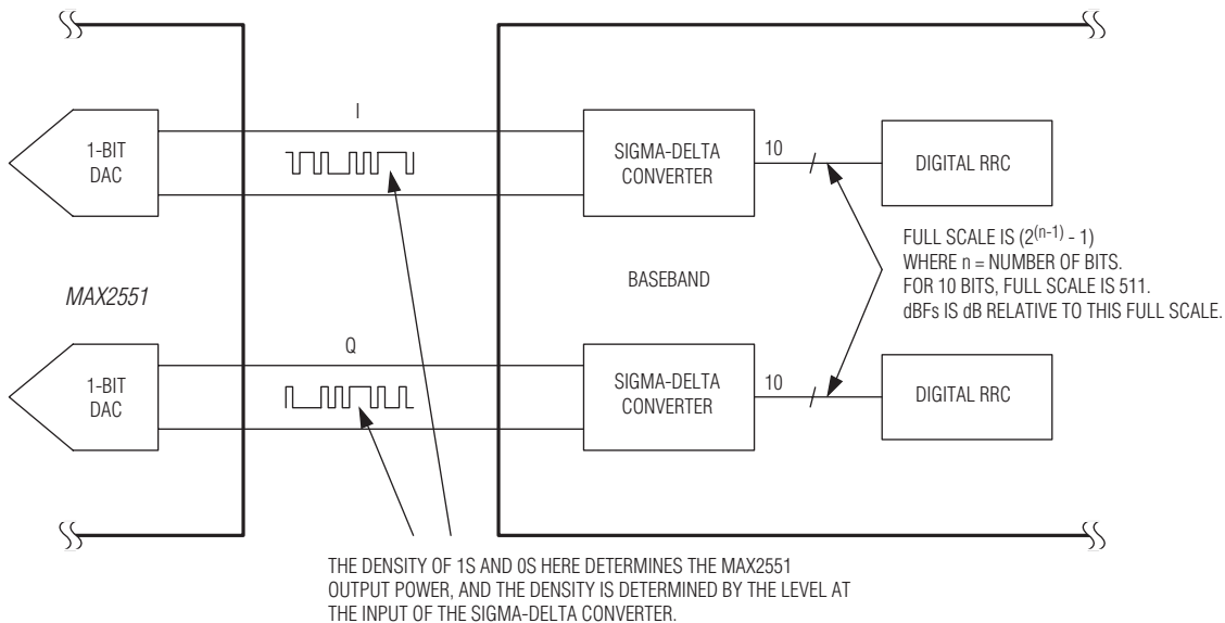
Figure 2. Baseband Input Example
