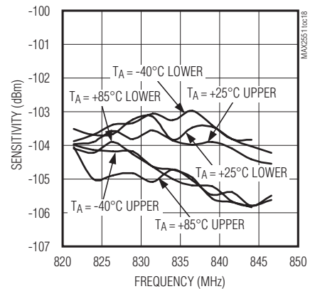
RXIN3 SENSITIVITY vs. FREQUENCY WITH -28dBm ADJACENT CHANNEL INTERFERENCE LNA GAIN = MAX, PGA GAIN = 3
