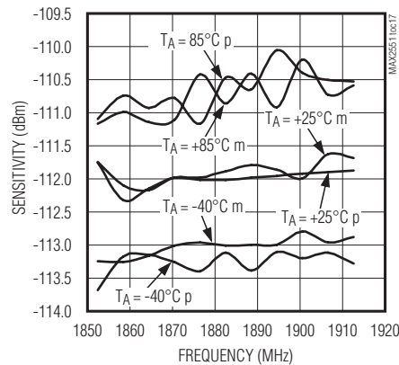
RXIN1 SENSITIVITY vs. FREQUENCY WITH -28dBm ADJACENT CHANNEL INTERFERENCE LNA GAIN = MID, PGA GAIN = 6
