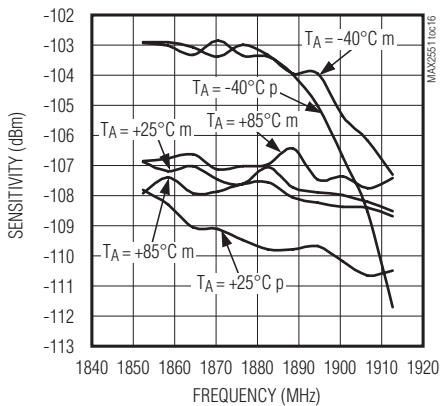
RXIN3 SENSITIVITY vs. FREQUENCY WITH -28dBm ADJACENT CHANNEL INTERFERENCE LNA GAIN = MID, PGA GAIN = 6
