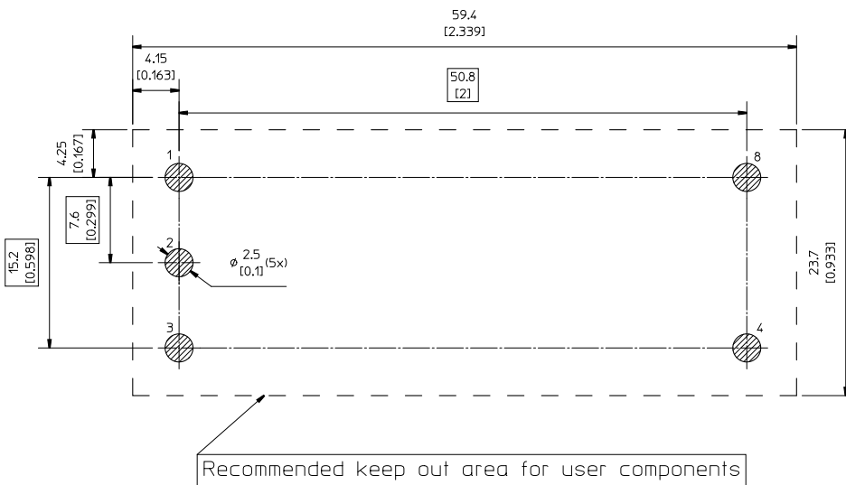
RECOMMENDED FOOTPRINT - TOP VIEW
