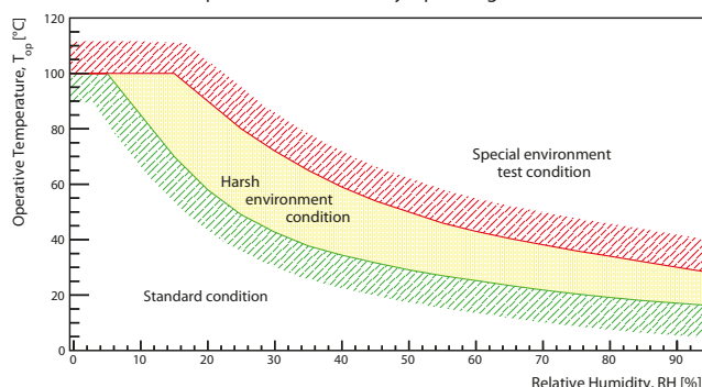
Temperature and Humidity Operating Reference
