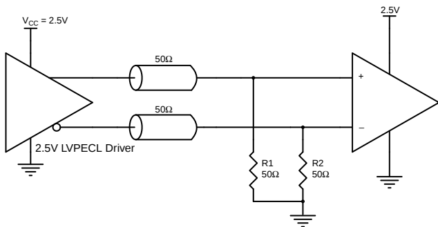
Figure 5C. 2.5V LVPECL Driver Termination Example
