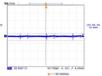
High Line, Full Load Ripple noise=18.4mV
