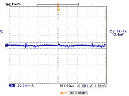
High Line, Full Load Ripple noise=12.4mV
