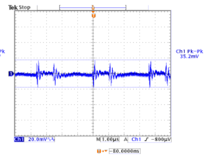
High Line, Full Load Ripple noise=35.2mV
