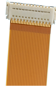
Premo-Flex Etched Polyimide Jumpers with Easy-On BackFlip FPC Connector, Pitch, Series 502598
