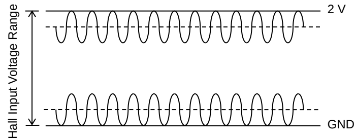
Figure 25. Hall Input Voltage Range
