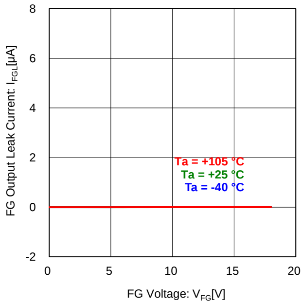
Figure 13. FG Output Leak Current vs FG Voltage ( V_{CC} = 12\text{ V} )
