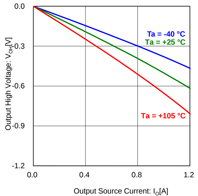
Figure 2. Output High Voltage vs Output Source Current ( V_{CC} = 12\text{ V} )
