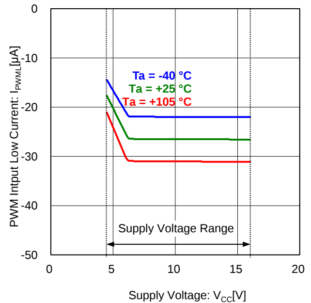
Figure 8. PWM Input Low Current vs Supply Voltage ( V_{PWM} = 0\text{ V} )
