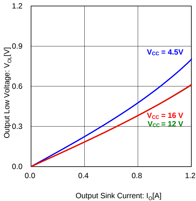
Figure 5. Output Low Voltage vs Output Sink Current ( T_a = 25^\circ\text{C} )
