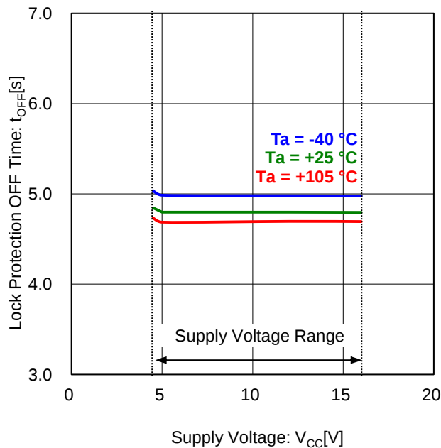
Figure 15. Lock Protection OFF Time vs Supply Voltage
