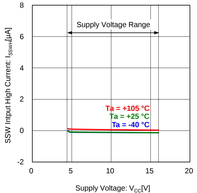
Figure 16. SSW Input High Current vs Supply Voltage ( V_{SSW} = 3.3\text{ V} )
