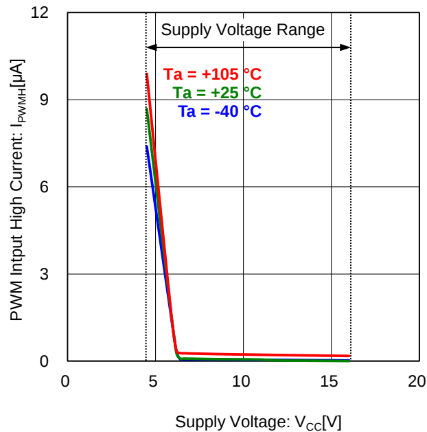
Figure 7. PWM Input High Current vs Supply Voltage ( V_{PWM} = 5\text{ V} )
