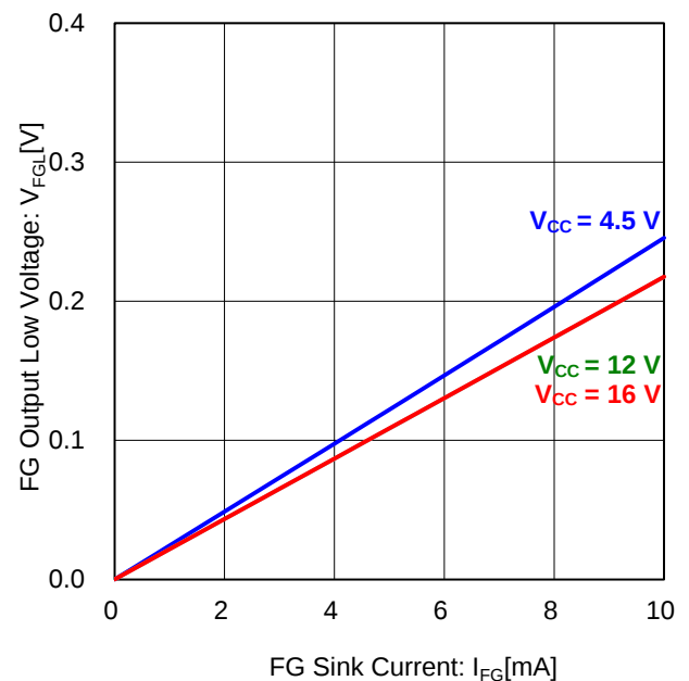
Figure 12. FG Output Low Voltage vs FG Sink Current ( T_a = 25\text{ }^{\circ}\text{C} )
