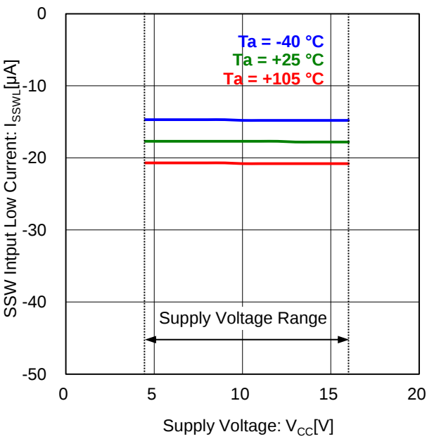
Figure 17. SSW Input Low Current vs Supply Voltage ( V_{SSW} = 0\text{ V} )
