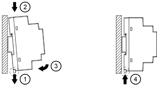
Fig. 2.1 Mounting
