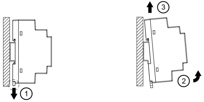
Fig. 2.2 Dismounting
