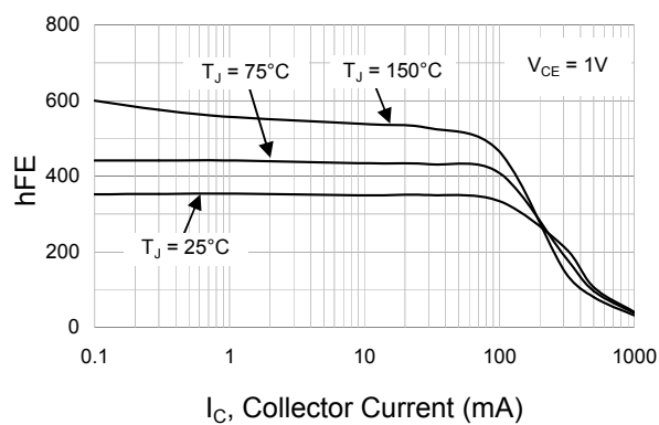
Fig.5 BC817-40W : DC Current Gain
