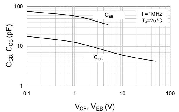
Fig.6 Typical Capacitance
