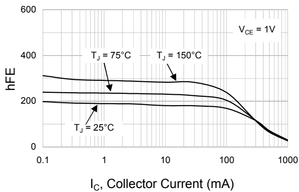
Fig.3 BC817-16W : Typical DC Current Gain
