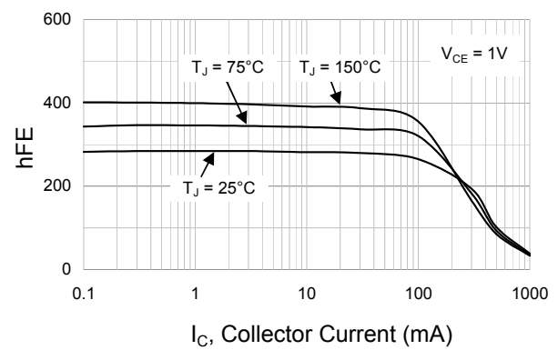
Fig.4 BC817-25W : Typical DC Current Gain
