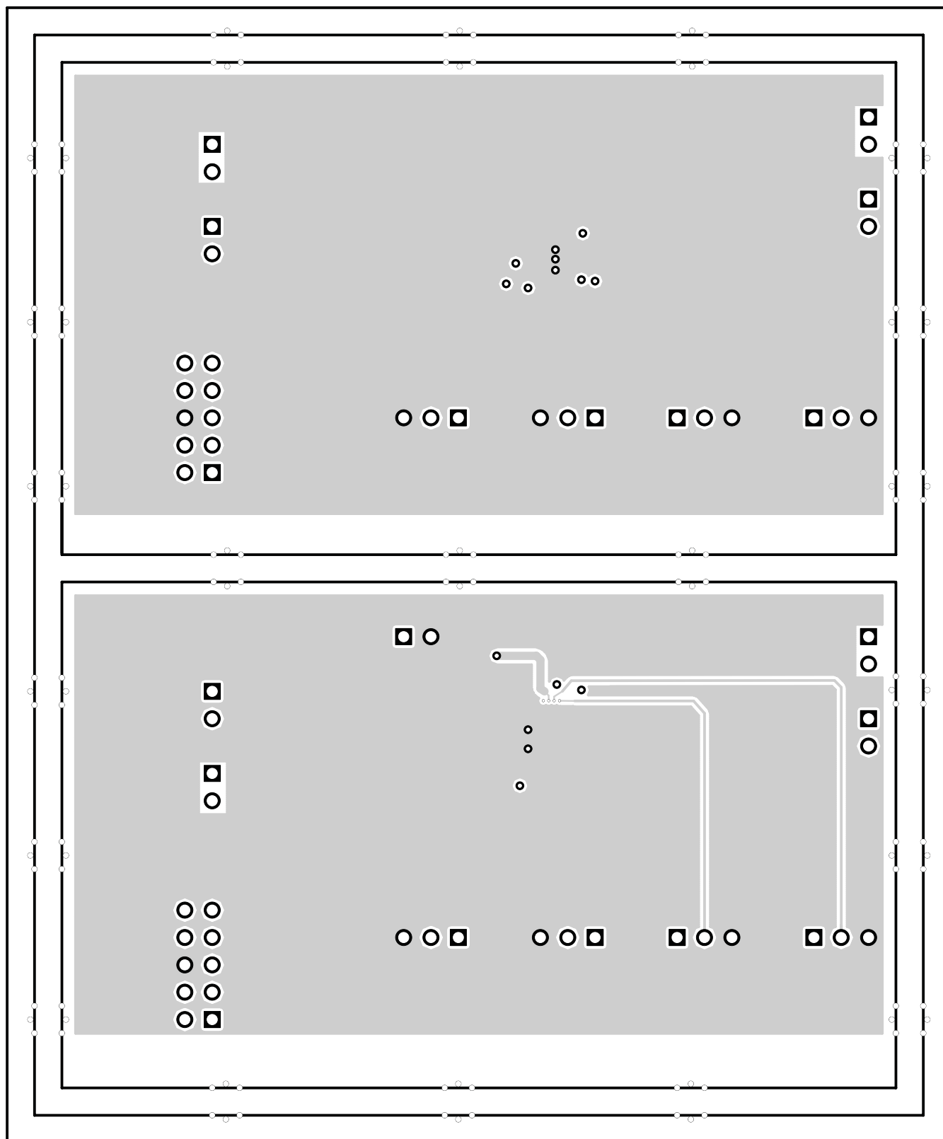
Figure 11. Layer 2 Routing
