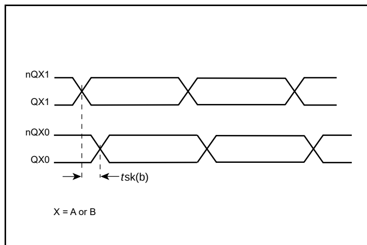
Bank Skew
