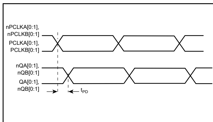
Propagation Delay
