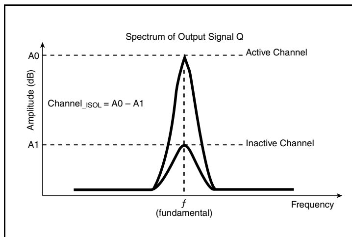
Channel Isolation
