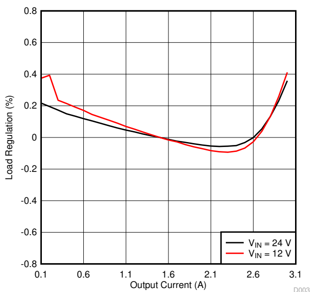
Figure 2-3. TPS54302EVM-716 Load Regulation
