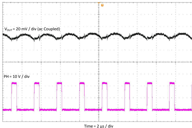
Figure 2-6. TPS54302EVM-716 Output Ripple, I_{OUT} = 3 A
