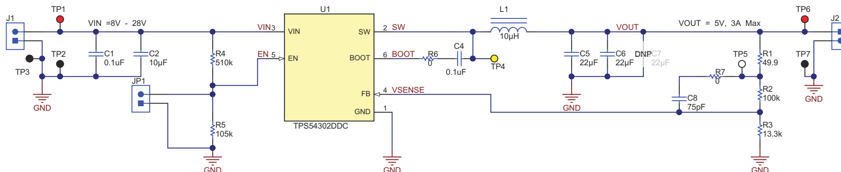
Figure 4-1. TPS54302EVM-716 Schematic
