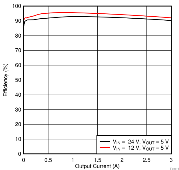
Figure 2-1. TPS54302EVM-716 Efficiency
