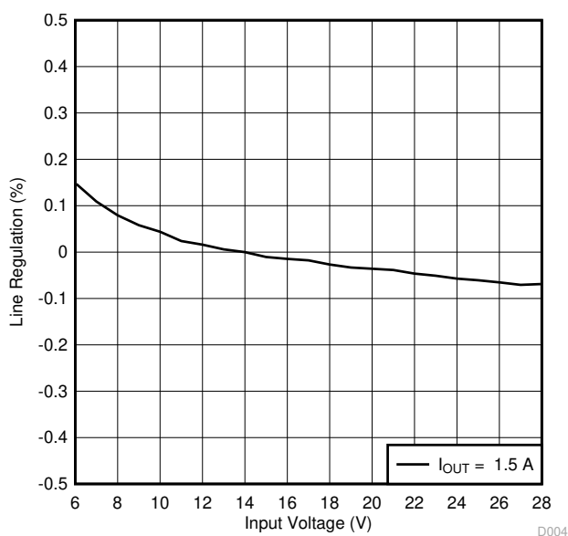
Figure 2-4. TPS54302EVM-716 Line Regulation
