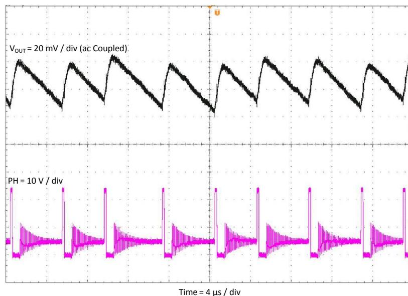
Figure 2-7. TPS54302EVM-716 Output Ripple, I_{OUT} = 100 mA
