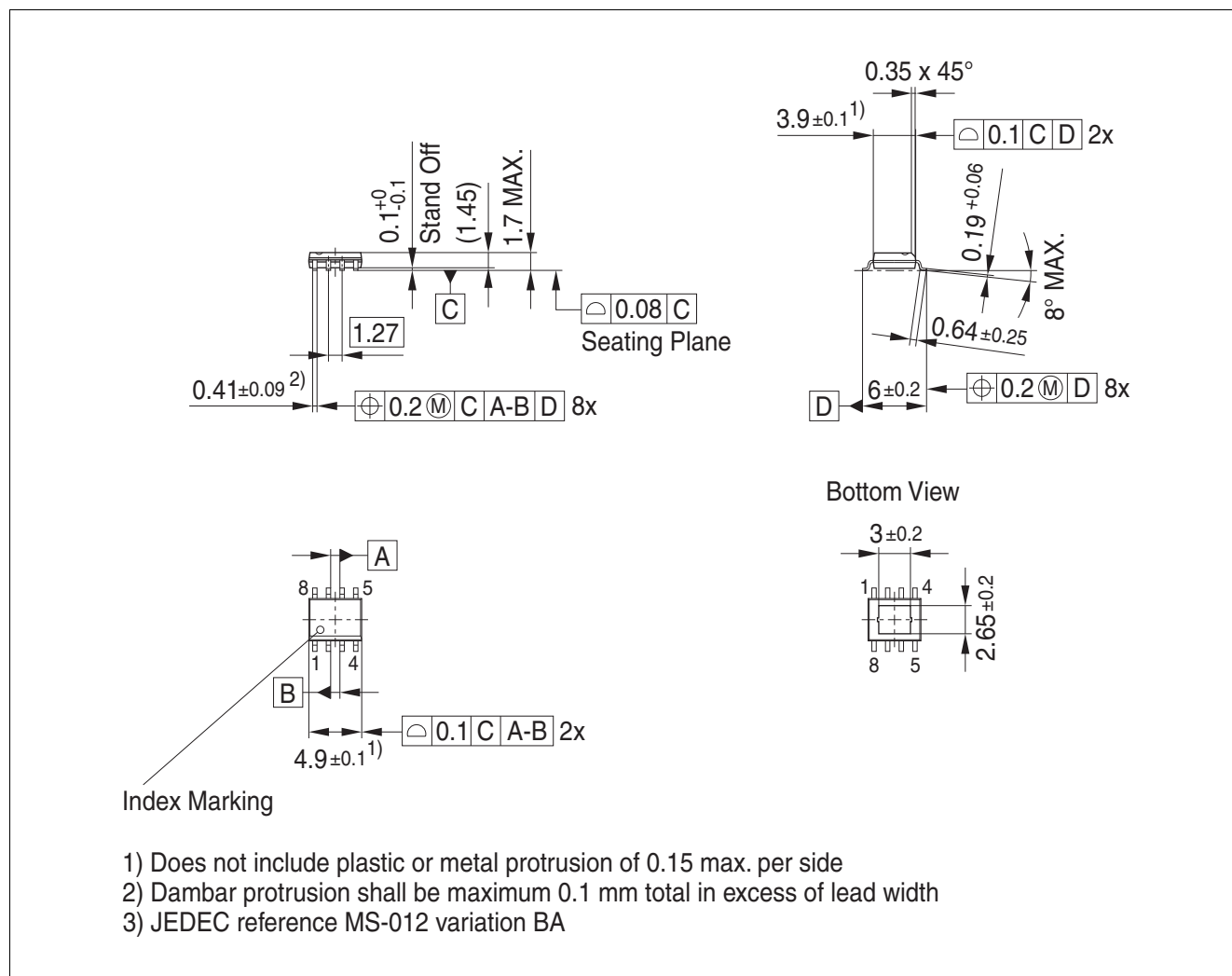
Figure 5 PG-DSO8-EP
