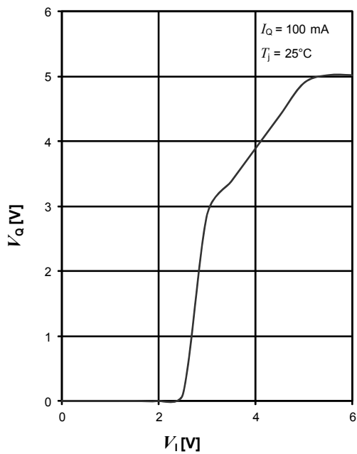
Output Voltage V_O versus Input Voltage V_I (TLF80511EJV50)
