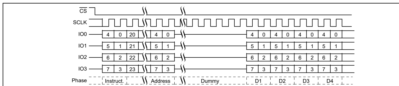
Figure 53 ECCRD (19h), Quad All Mode, CR2[7] = 0, command sequence
