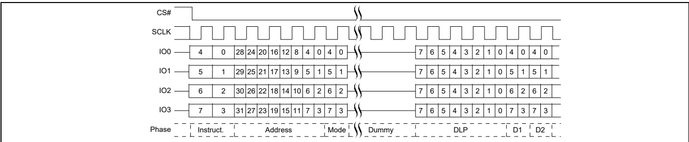
Figure 15 DDR Quad I/O Read in QPI mode
