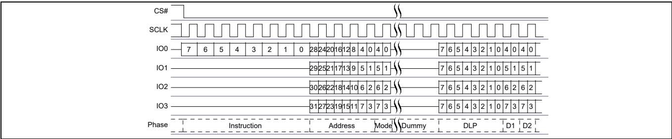
Figure 14 DDR Quad I/O Read
