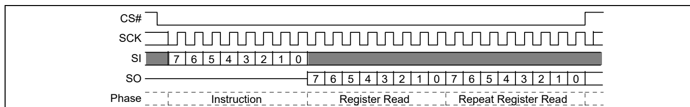
Figure 56 DLP Read (DLPRD) command sequence
