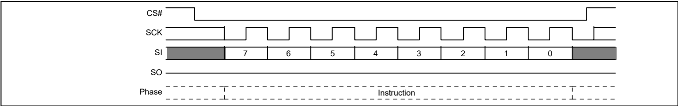
Figure 50 Clear Status Register (CLSR) command sequence
