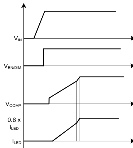
Figure 2: Soft-Start Process
