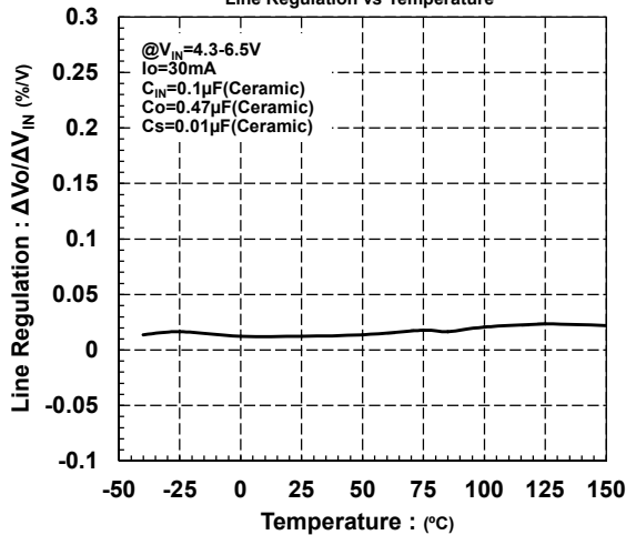
NJM12888_3.3V
