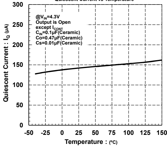
NJM12888_3.3V
