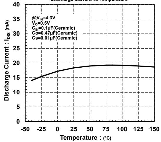
NJM12888_3.3V
