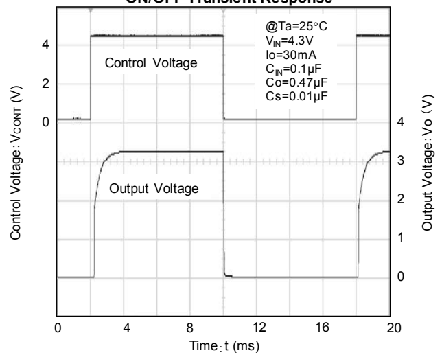
NJM12888_3.3V ON/OFF Transient Response
