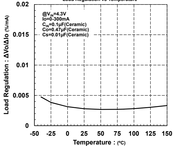
NJM12888_3.3V
