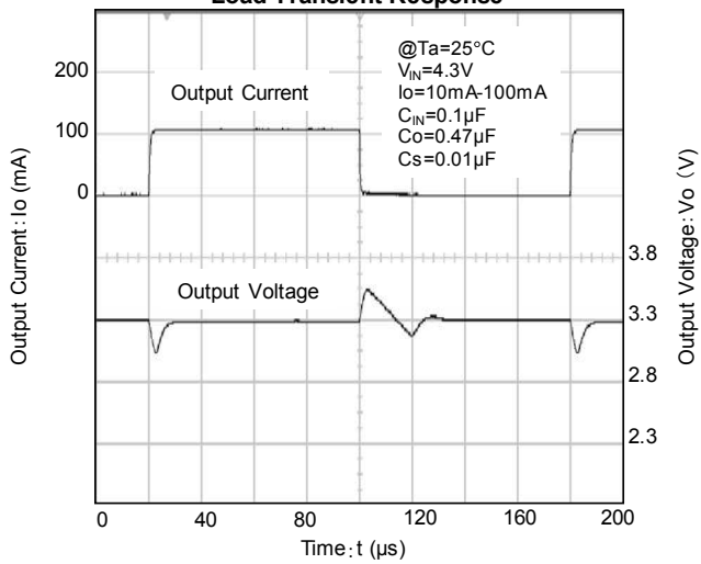
NJM12888_3.3V Load Transient Response
