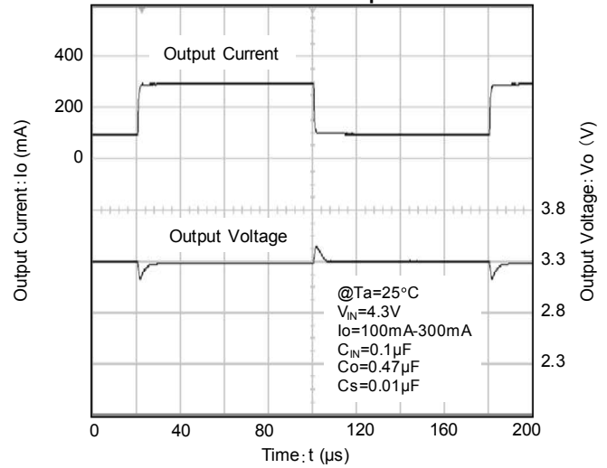
NJM12888_3.3V Load Transient Response
