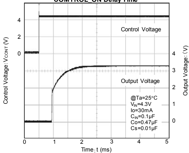
NJM12888_3.3V CONTROL_ON Delay Time
