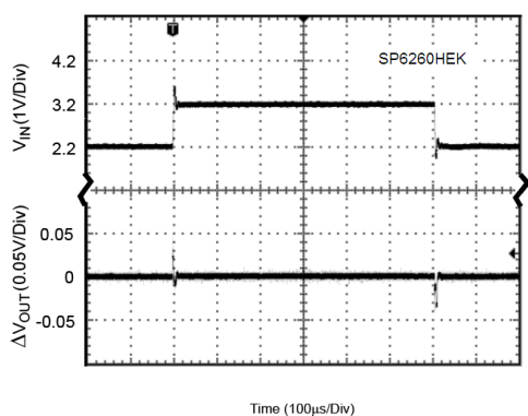
Fig. 19: Line Transient SP6260HEK (1.2V) (Conditions: I_{\text{OUT}} = 30\text{mA} , C_{\text{IN}} = 1\mu\text{F} , C_{\text{OUT}} = 1\mu\text{F} )
