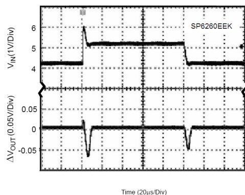
Fig. 20: Line Transient SP6260EEK (3.0V) (Conditions: I_{\text{OUT}} = 30\text{mA} , C_{\text{IN}} = 1\mu\text{F} , C_{\text{OUT}} = 1\mu\text{F} )
