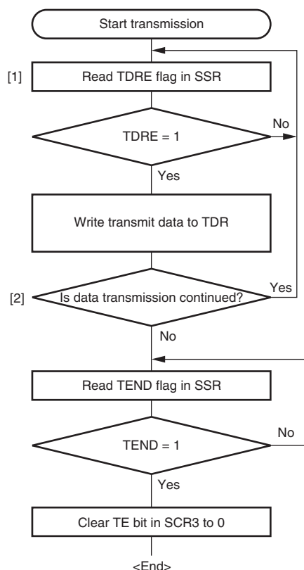
Figure 20.11 Sample Flowchart for Data Transmission (Clocked Synchronous Mode)
