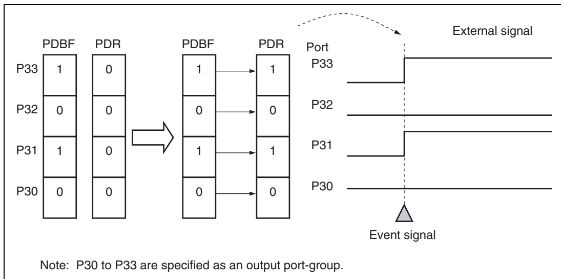
Figure 12.5 Event Linkage related to Output Port-Groups
