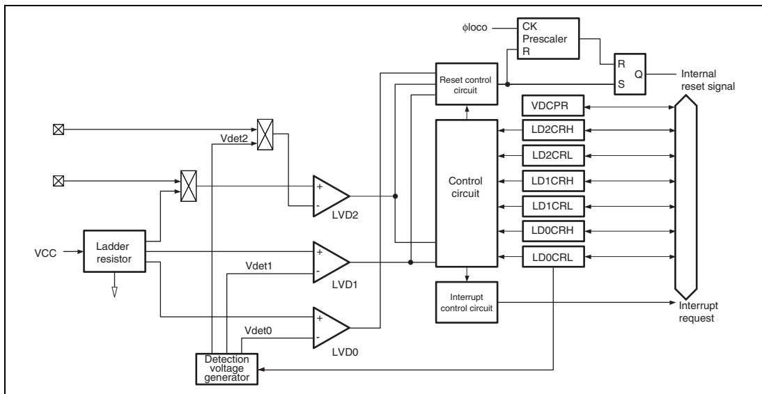
Figure 26.1 Block Diagram of Low-Voltage Detection Circuits
