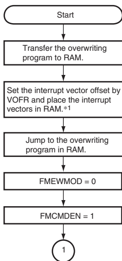
Flow of initialization for EW1 mode*1
