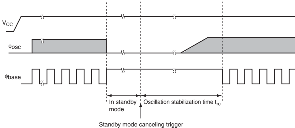
Figure 28.3 Oscillation Stabilization Time Timing
