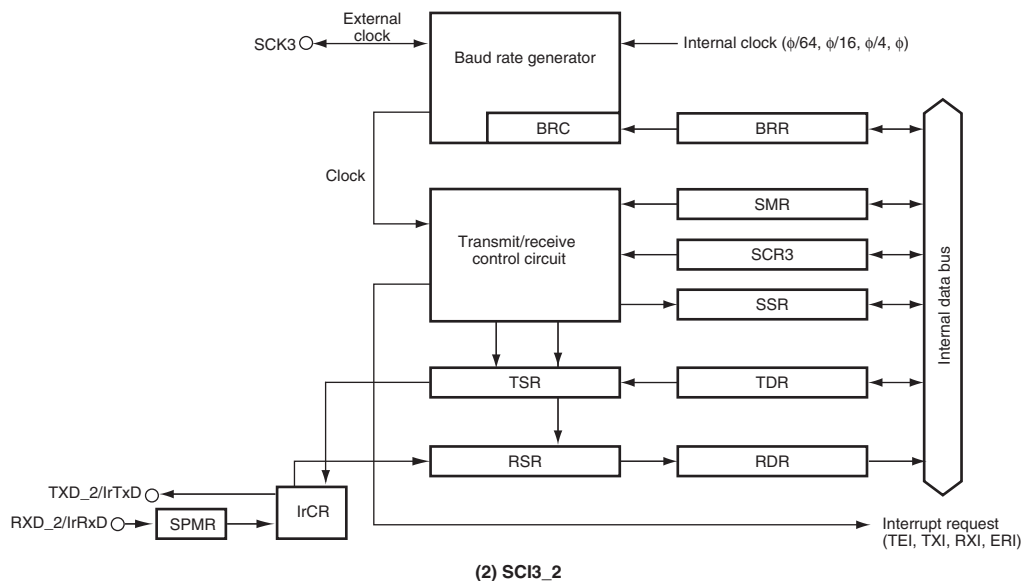
Figure 20.1 Block Diagram of SCI3
