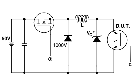
Fig. 13a - Clamped Inductive Load Test Circuit
