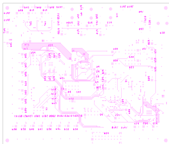
Figure 19. EVAL-ADAU1860EBZ Layer 4, Bottom Side
