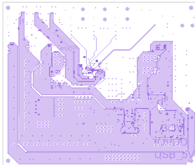
Figure 18. EVAL-ADAU1860EBZ Layer 3, Power Plane
