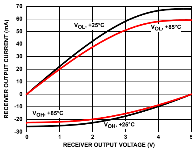
FIGURE 13. RECEIVER OUTPUT CURRENT vs RECEIVER OUTPUT VOLTAGE
