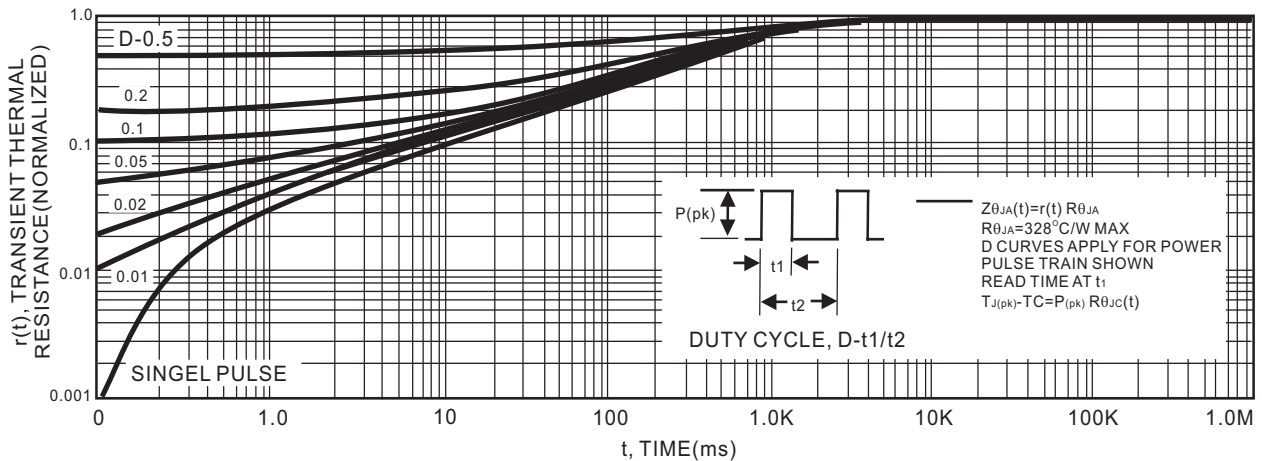
Figure 7. Thermal Response
