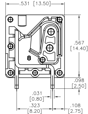
WITHOUT COVER
