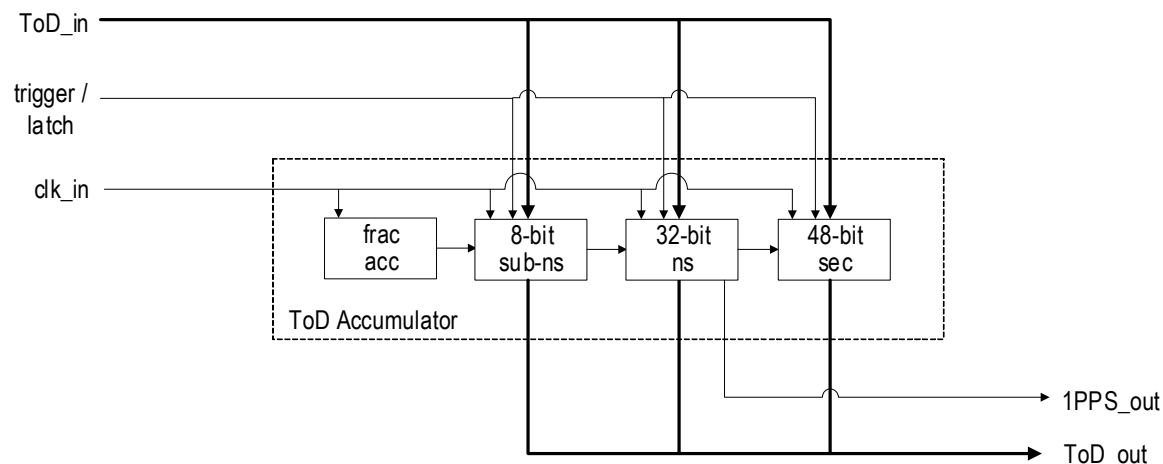
Figure 34. ToD Accumulator
