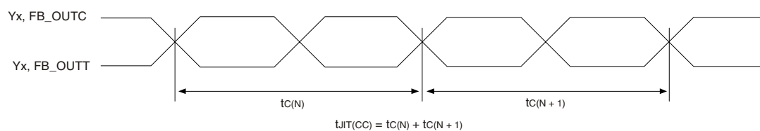
Figure 3: Cycle-to-Cycle Jitter
