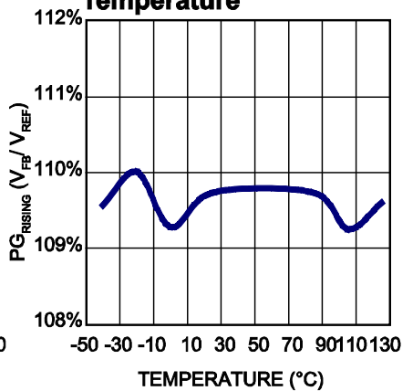
PG Rising Threshold (VFB Falling) vs. Temperature
