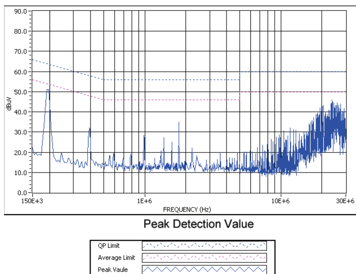
Graph 2. Conducted emissions performance, Negative Line, CISPR 22, Class B, 48 Vin, full load
