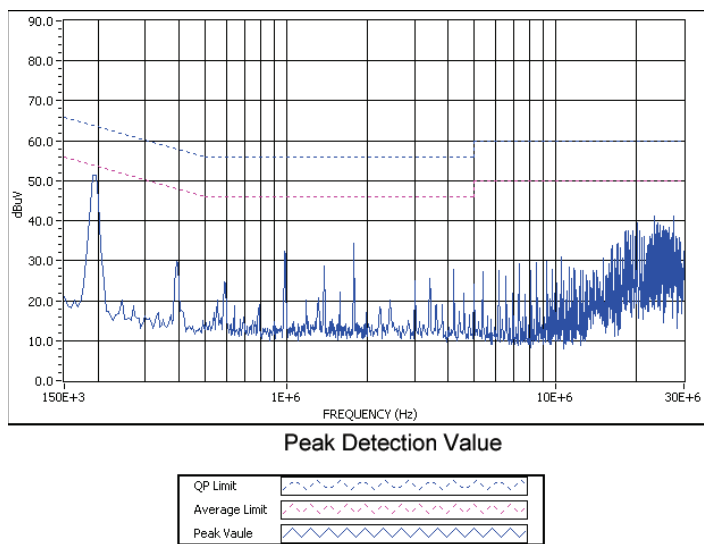
Graph 1. Conducted emissions performance, Positive Line, CISPR 22, Class B, 48 Vin, full load
