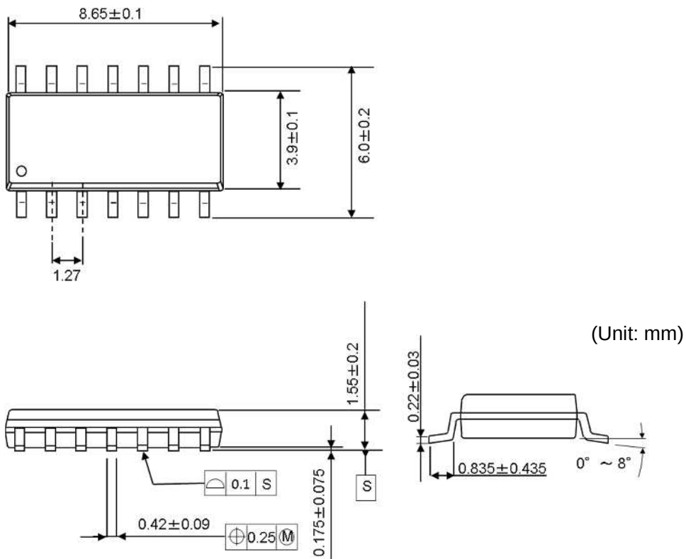
SOP14 Package
