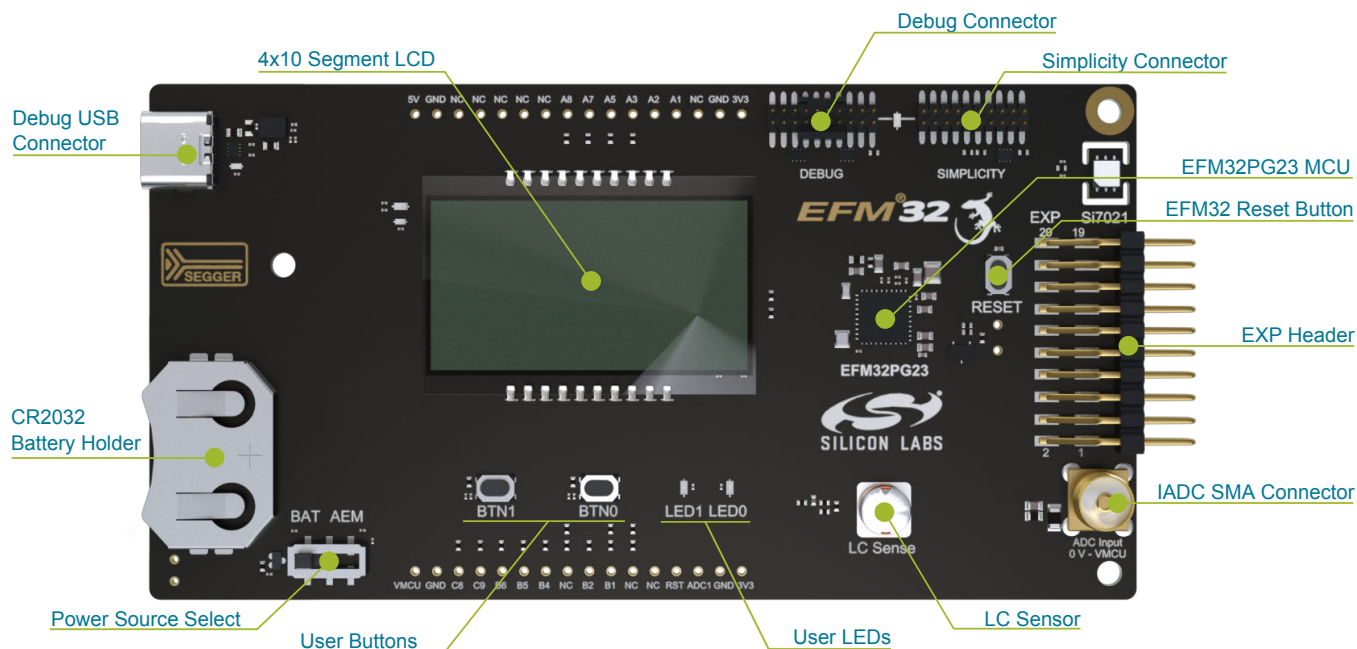
Figure 3.1. PG23 Pro Kit Hardware Layout
