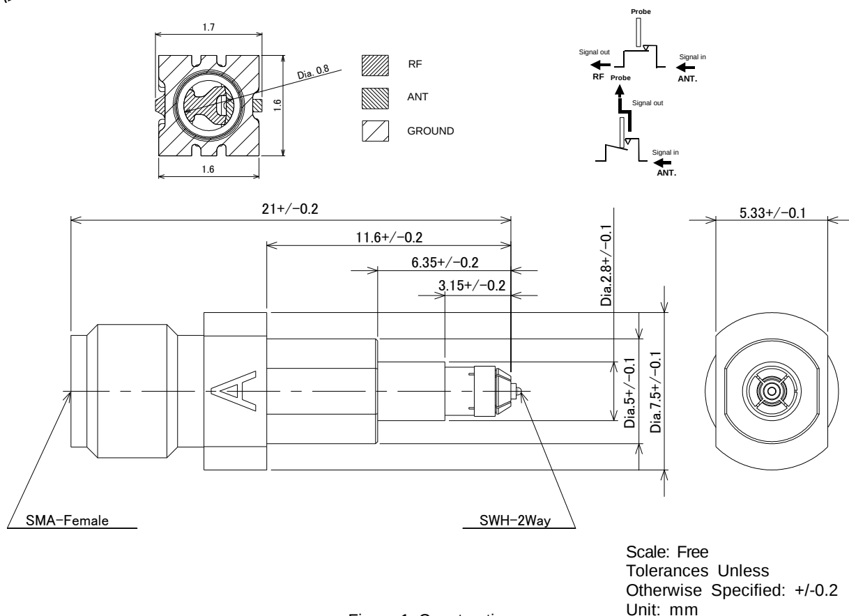
Figure.1 Construction
