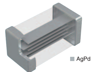
Fig.2 Internal structure of the multilayer chip Thermistors
