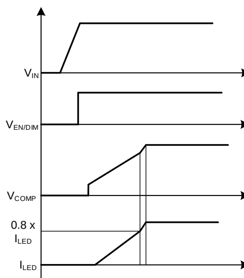
Figure 2: Soft Start
