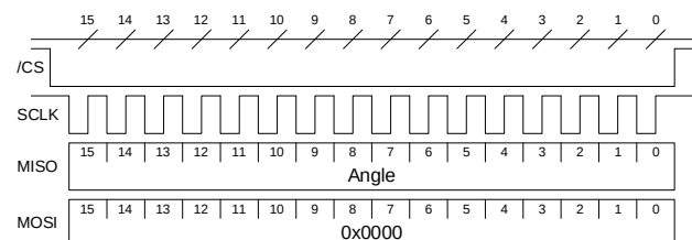
Figure 10: Full 16-Bit SPI Angle Reading Diagram
