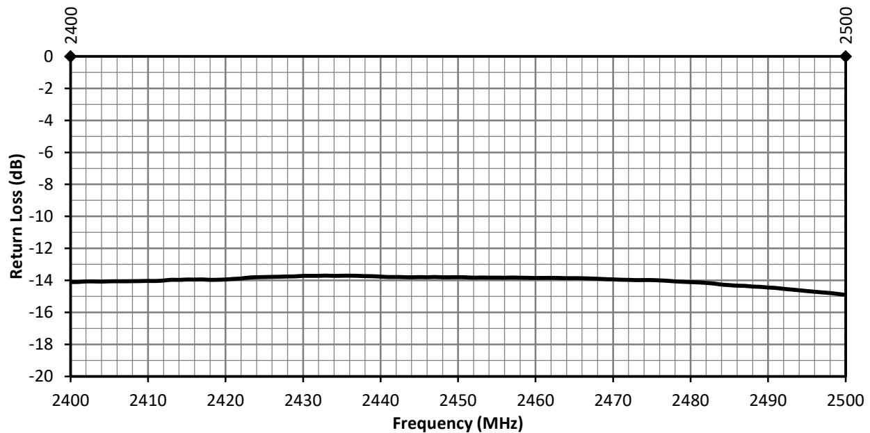
Figure 6. ANT-2.4-WRT Return Loss, Free Space
