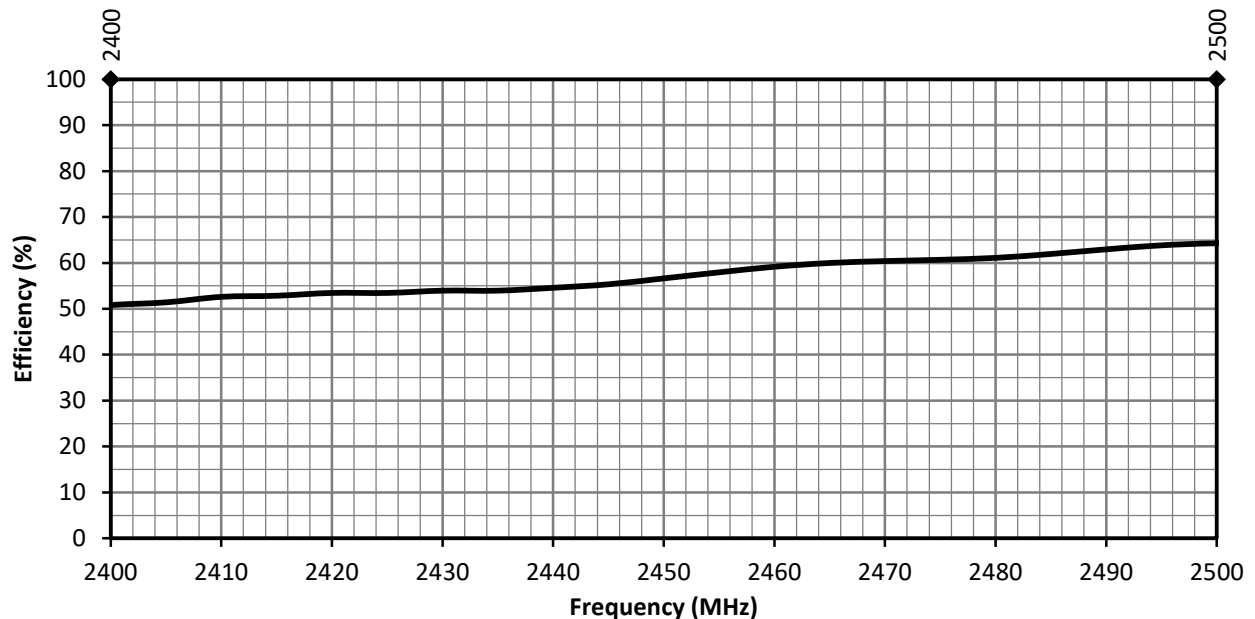
Figure 16. ANT-2.4-WRT Antenna Radiation Efficiency at Center of Ground Plane
