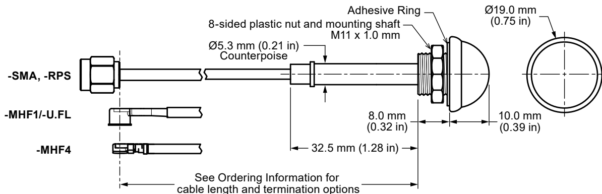
Figure 1. ANT-2.4-WRT Series Antenna Dimensions
