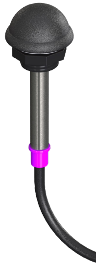
Figure 4. ANT-2.4-WRT in Free Space, No Ground Plane
