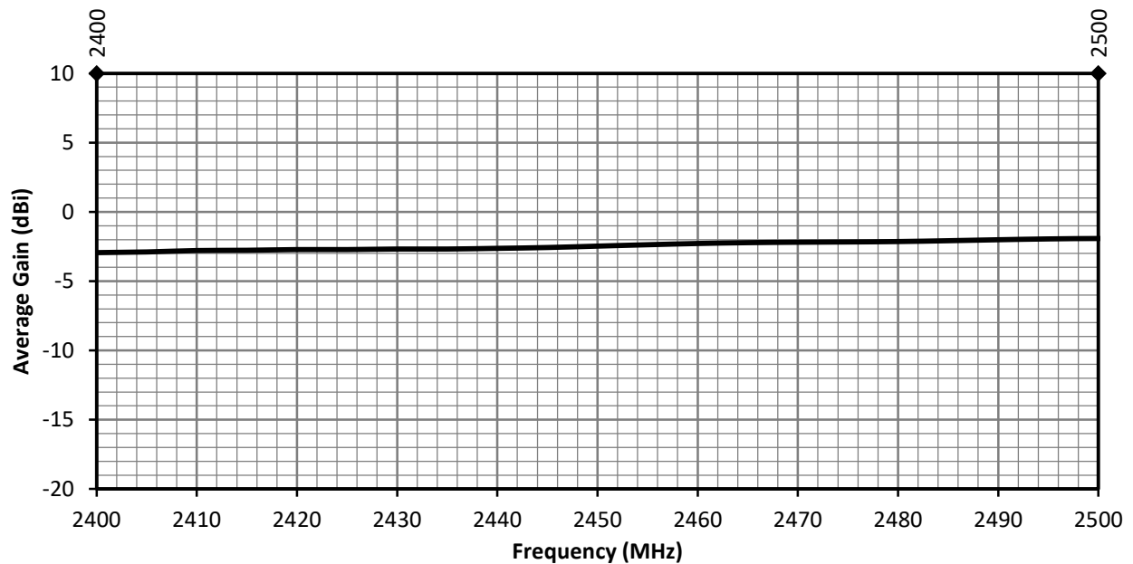
Figure 15. ANT-2.4-WRT Antenna Average Gain at Center of Ground Plane
