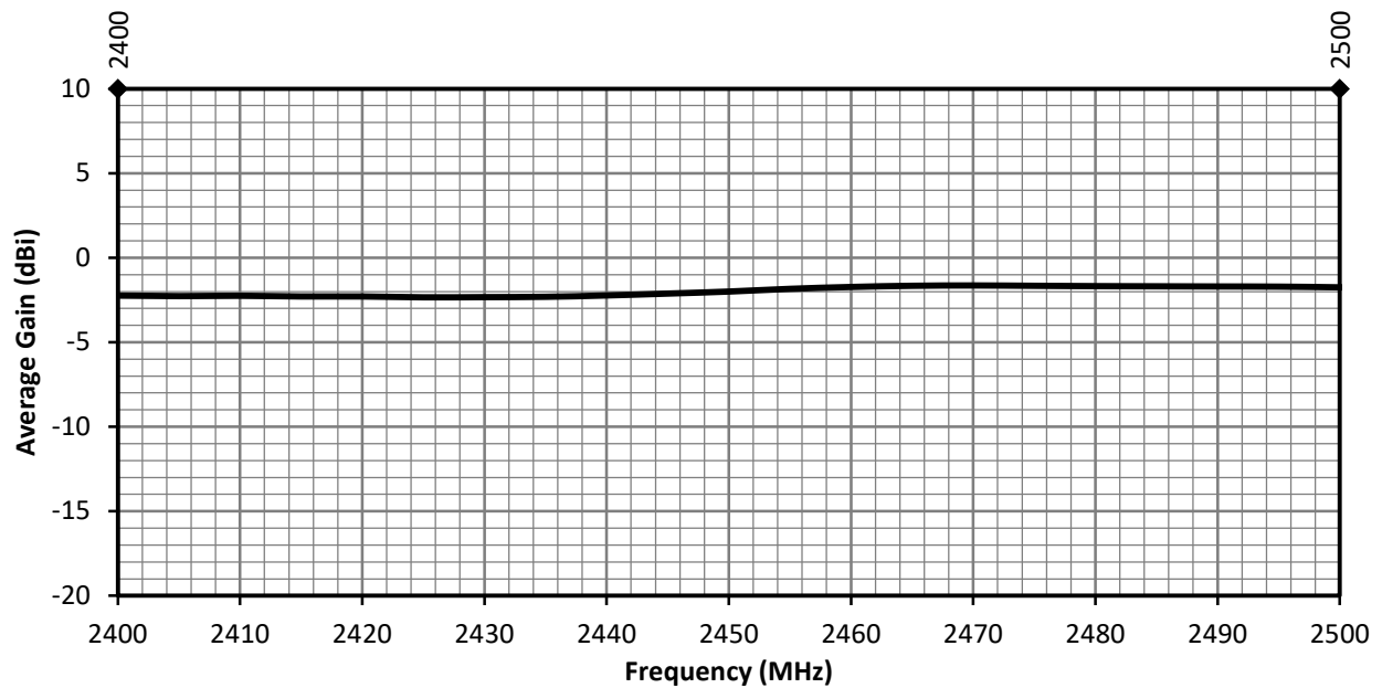
Figure 8. ANT-2.4-WRT Antenna Average Gain, Free Space
