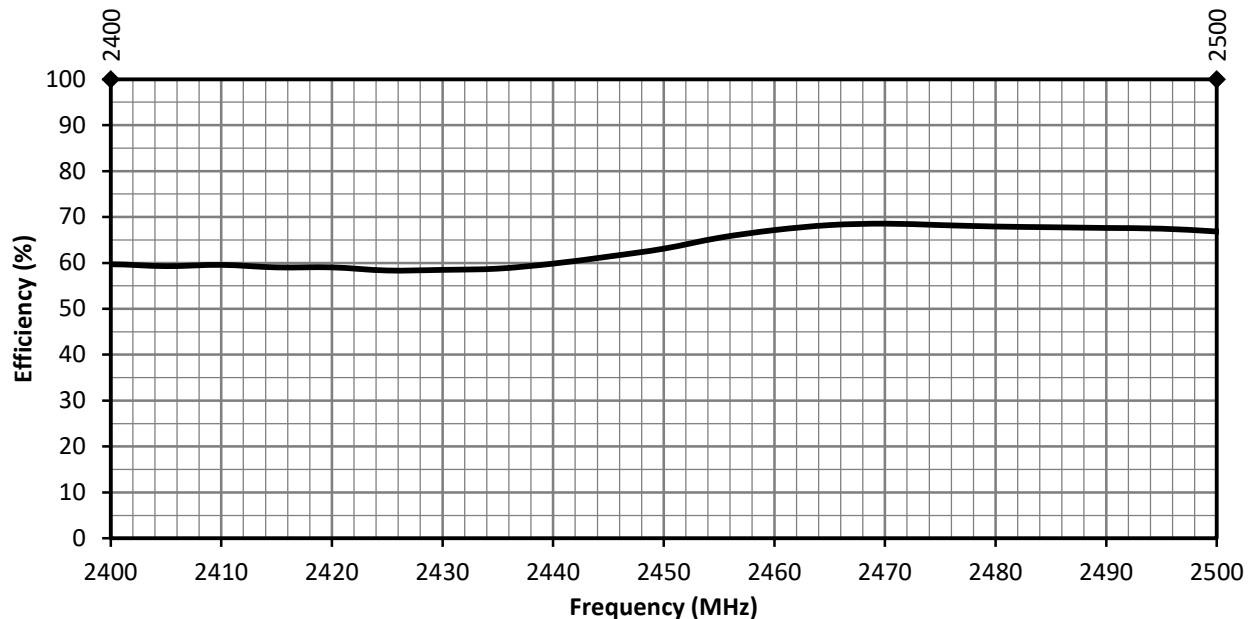
Figure 9. ANT-2.4-WRT Series Antenna Radiation Efficiency, Free Space
