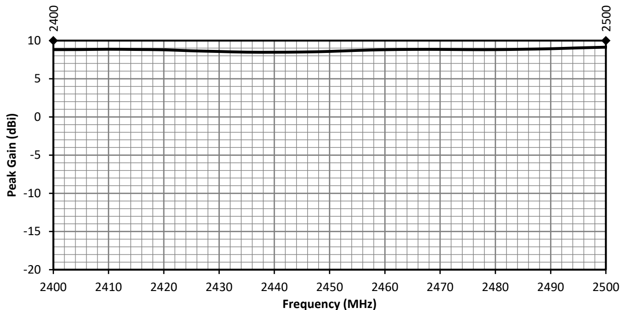
Figure 7. ANT-2.4-WRT Peak Gain, Free Space
