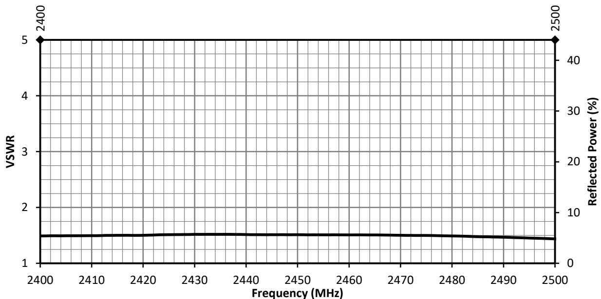
Figure 5. ANT-2.4-WRT VSWR, Free Space
