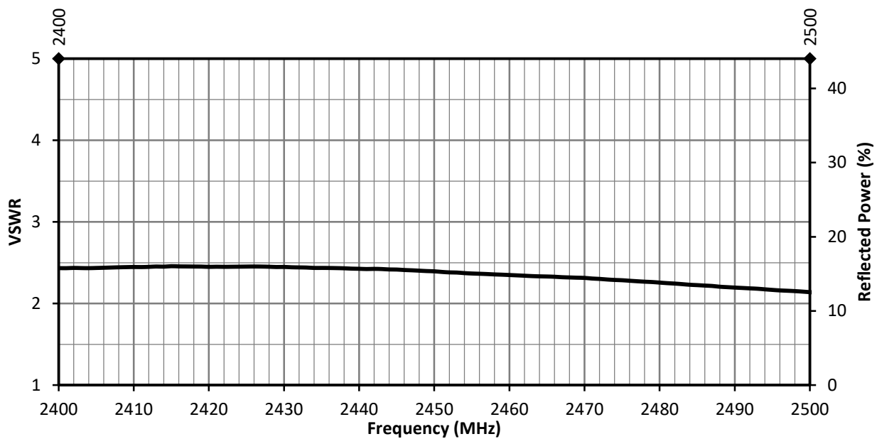
Figure 12. ANT-2.4-WRT Antenna VSWR at Center of Ground Plane
