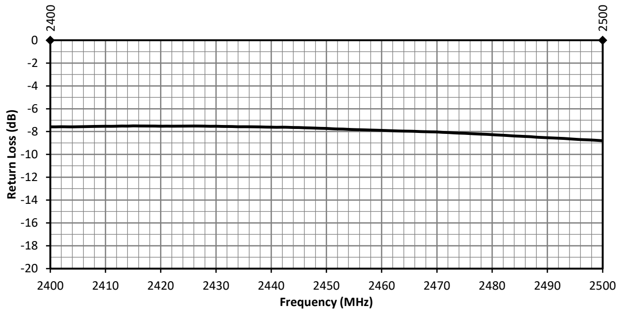
Figure 13. ANT-2.4-WRT Return Loss at Center of Ground Plane
