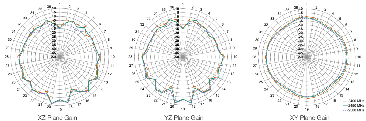
Figure 10. ANT-2.4-WRT Antenna Radiation Patterns, Free Space
