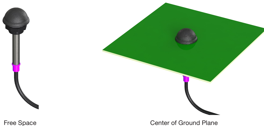
Figure 3. ANT-2.4-WRT Series Antenna Test Orientations
