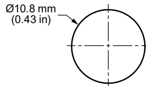
Figure 2. ANT-2.4-WRT Series Antenna Recommended Enclosure Mounting Dimensions
