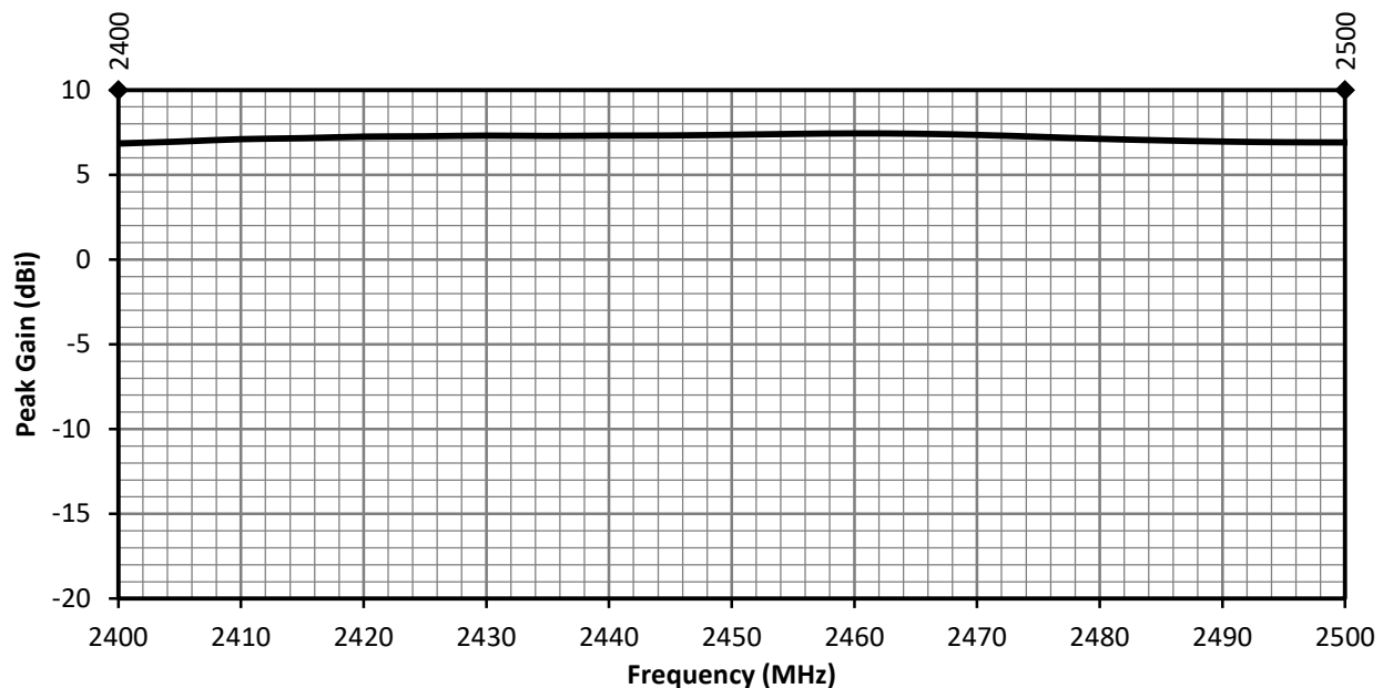
Figure 14. ANT-2.4-WRT Peak Gain at Center of Ground Plane
