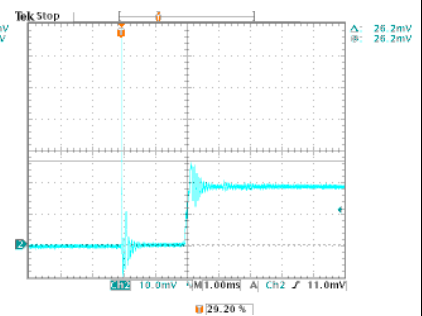
High Line, Full Load Inrush current=(26.2/10) x200mA=524mA
