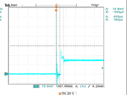
High Line, Full Load Duration: 400uS
