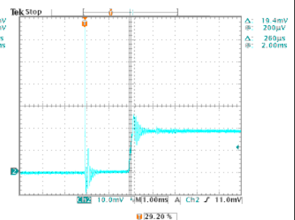
High Line, Full Load Duration: 260uS
