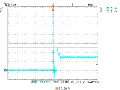
High Line, Full Load Inrush current=(25.2/10) x200mA=504mA
