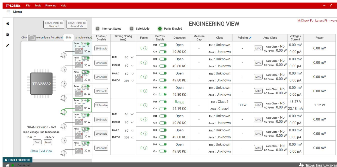
Figure 4-4. Device Configuration and Port Telemetry Page
