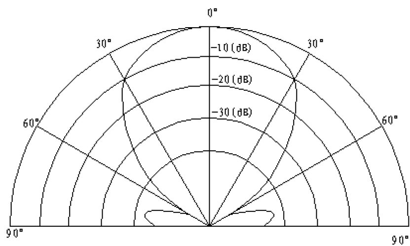
Directivity
