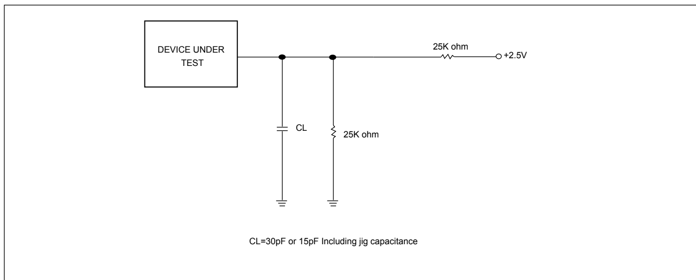
Figure 30. OUTPUT LOADING
