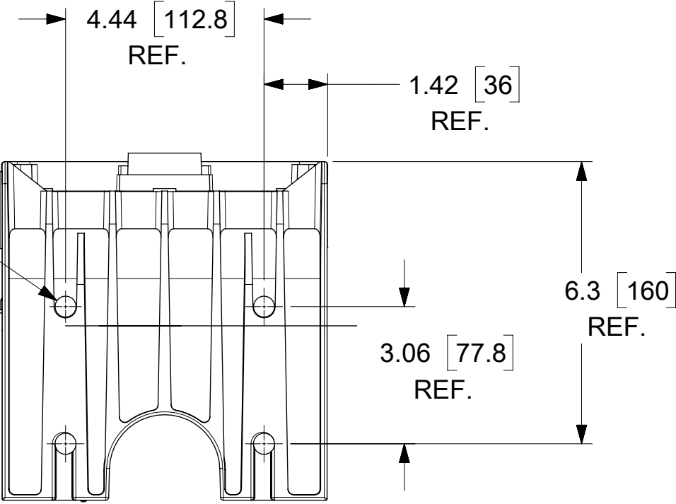
BOTTOM VIEW
