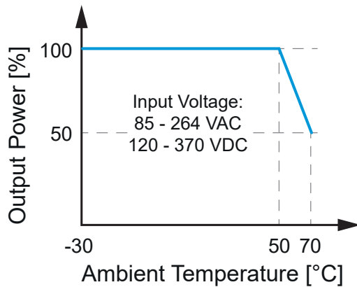
Figure 1. Temperature Derating Curve
