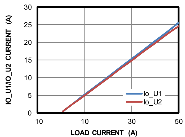
Current Sharing
