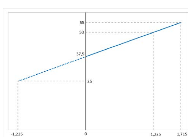
Desired output voltage vs. adjust voltage, R_{adj} = 2 \text{ k}\Omega
