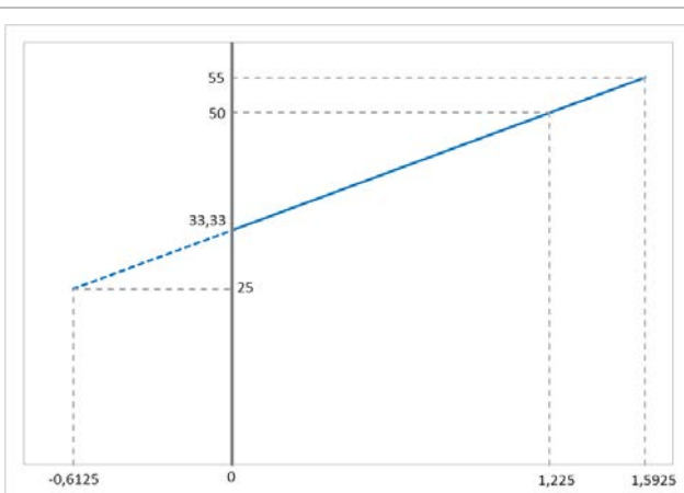
Desired output voltage vs. adjust voltage, R_{adj} = 1 \text{ k}\Omega
