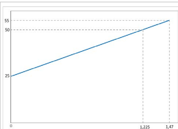
Desired output voltage vs. adjust voltage, R_{adj} = 0 \text{ k}\Omega
