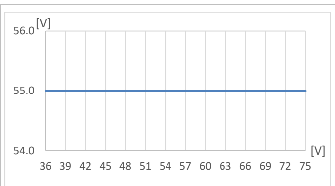
Max adjustable output voltage vs. input voltage at T_{P1} = +25^{\circ}\text{C}
