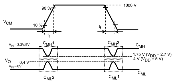
Fig. 12.6 Common-Mode Transient Immunity Test Circuit and Waveform
