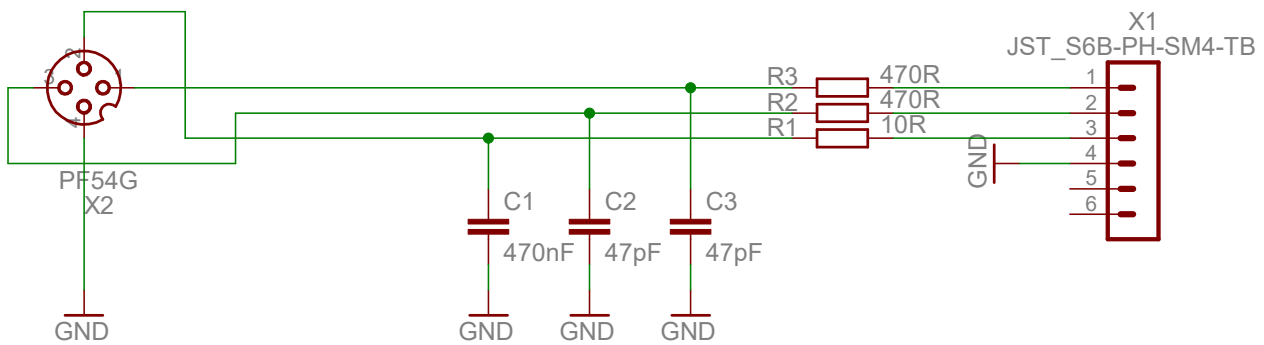
Figure 2: Part Schematics and Connections
