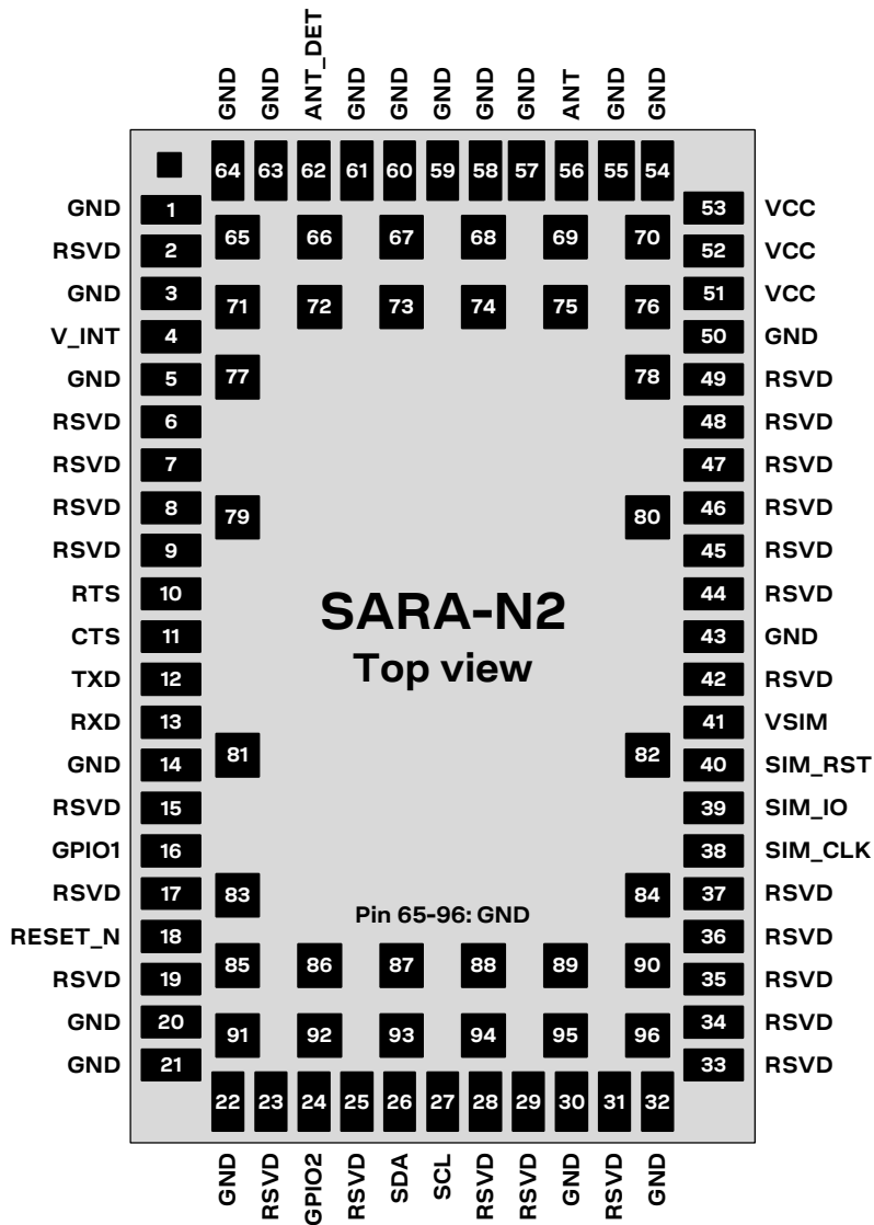
Figure 2: SARA-N2 series modules pin assignment
