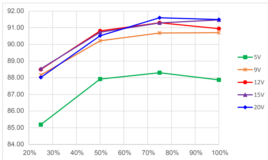
Figure 3. Efficiency @115 Vac
