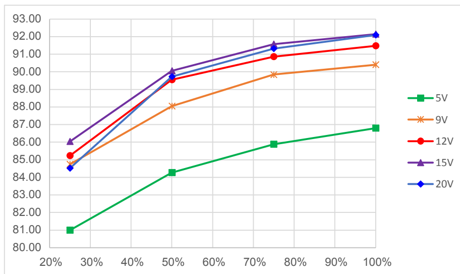
Figure 4. Efficiency @230Vac
