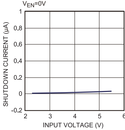
Shutdown Current vs. Input Voltage V EN =0V
