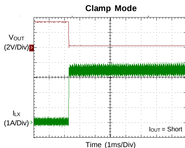
Figure 7. Clamp Mode
