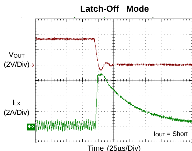
Figure 6. Latch-Off Mode Under Voltage Protection
